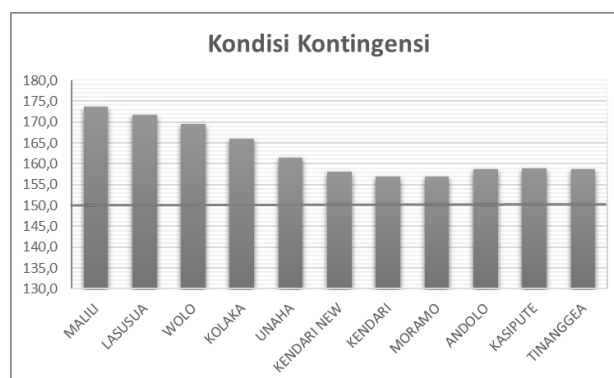
Figure 5. Busbar voltage under contingency conditions.
