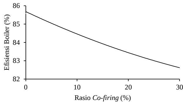
Figure 3. Boiler Efficiency (HHV) vs Co-firing Ratio
