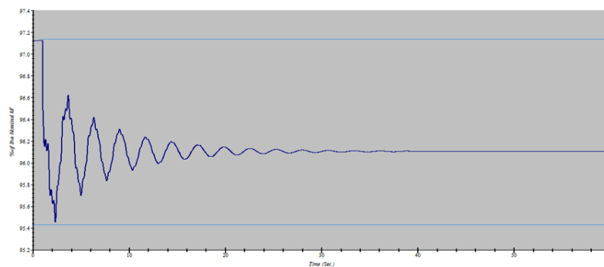
Figure 11. Voltage variation when FPV loss the supply 100%
